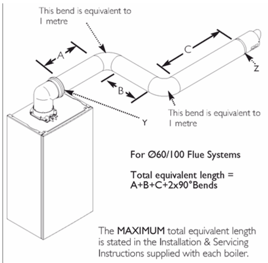
Horizontal Flue System Examples
