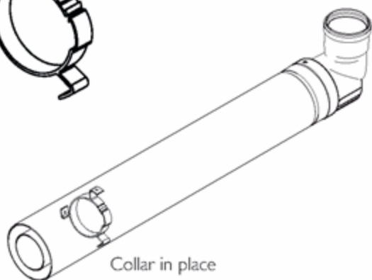
Centralising Collar
