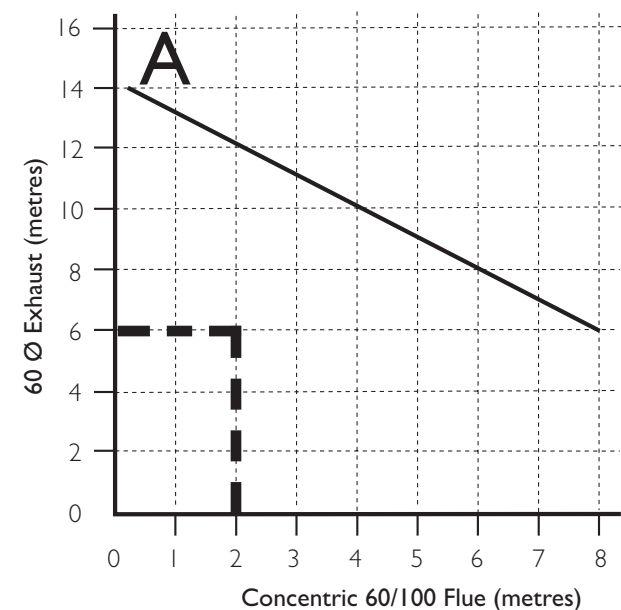
Example 3:- Flue Length - OK
