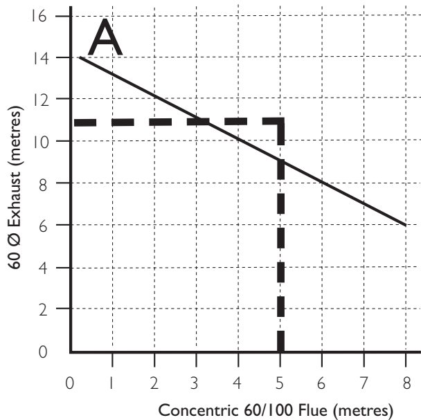
Example 1:- Flue Length - Not Permissible
