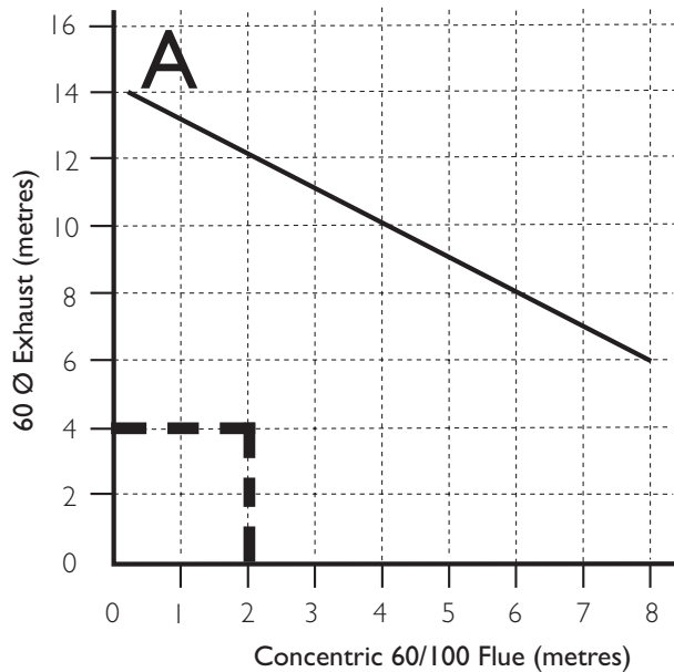
Example 2:- Flue Length - OK
