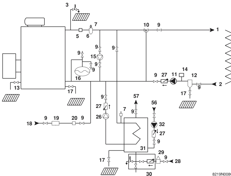
P 320 boiler with domestic hot water production using an independent tank
